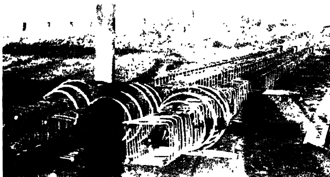
Fig. 192.—Reinforcement for Tapered "Collar" Piles, Kerse Bridge.
